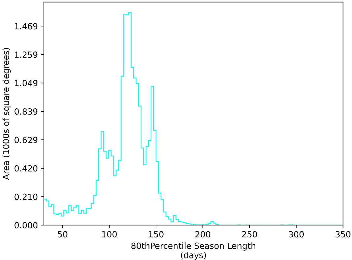
ddf_half_v3.4_10yrs All sky u band: 80thPercentile Season Length
