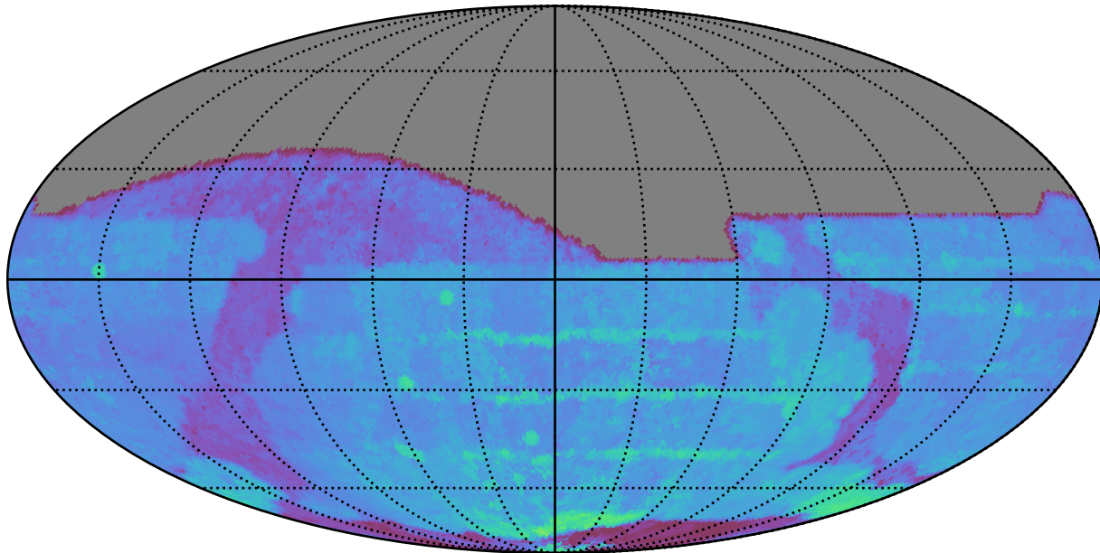
ddf_half_v3.4_10yrs All sky r band: 80thPercentile Season Length
