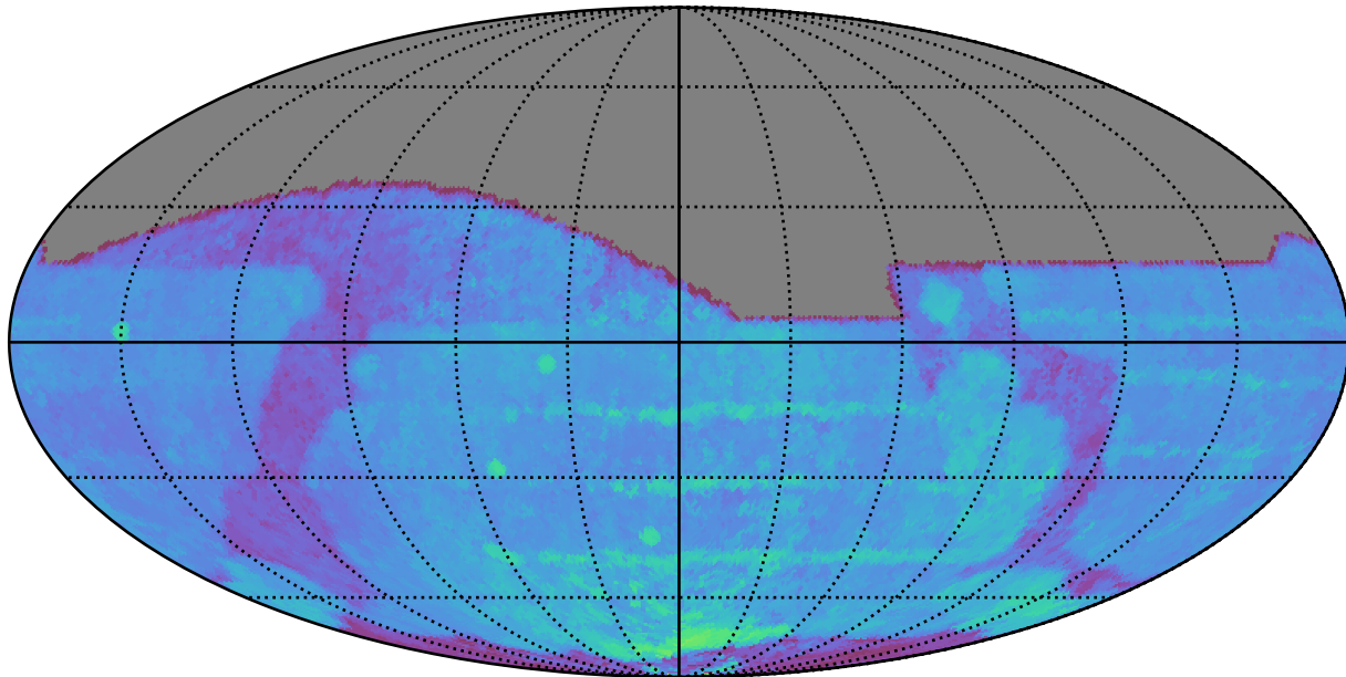
ddf_half_v3.4_10yrs All sky i band: 80thPercentile Season Length
