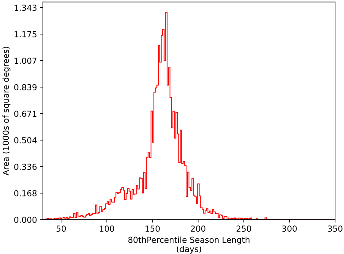
ddf_half_v3.4_10yrs All sky i band: 80thPercentile Season Length
