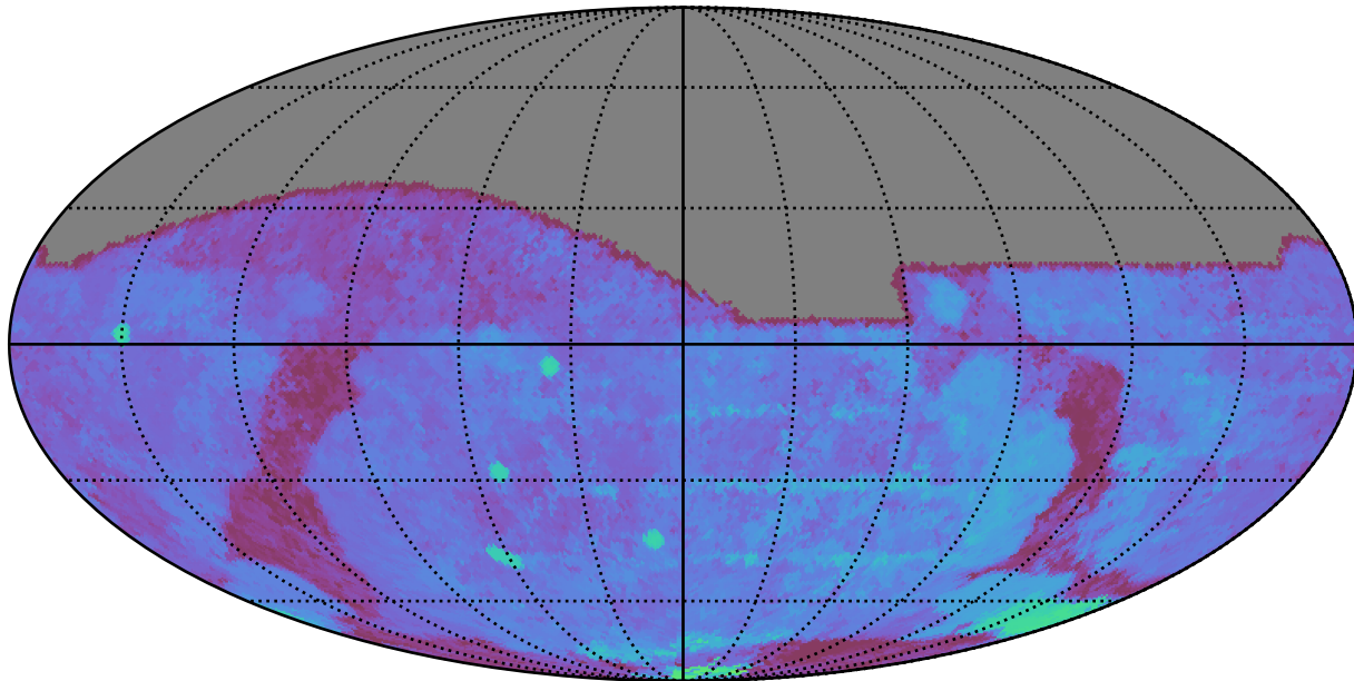
ddf_half_v3.4_10yrs All sky g band: 80thPercentile Season Length
