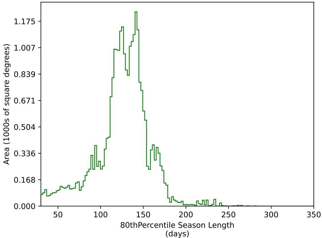
ddf_half_v3.4_10yrs All sky g band: 80thPercentile Season Length
