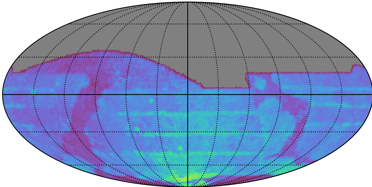
ddf_half_v3.4_10yrs All sky all bands: 80thPercentile Season Length
