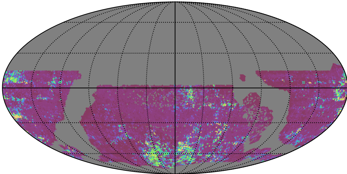
ddf_half_v3.4_10yrs WFD z band: 75th Percentile Intranight Timespan
