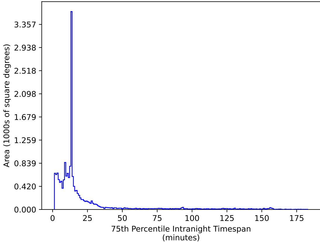
ddf_half_v3.4_10yrs WFD z band: 75th Percentile Intranight Timespan
