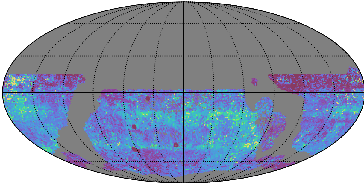
ddf_half_v3.4_10yrs WFD y band: 75th Percentile Intranight Timespan
