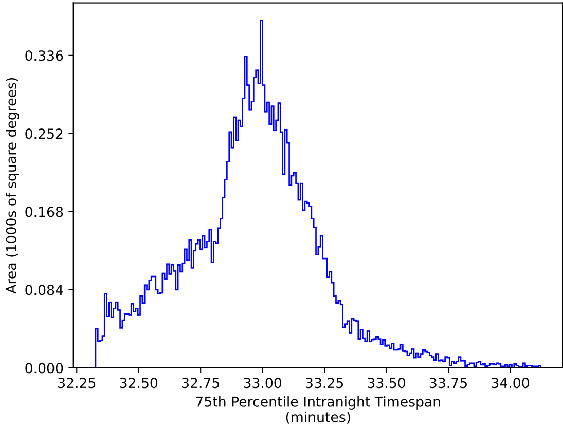
ddf_half_v3.4_10yrs WFD y band: 75th Percentile Intranight Timespan
