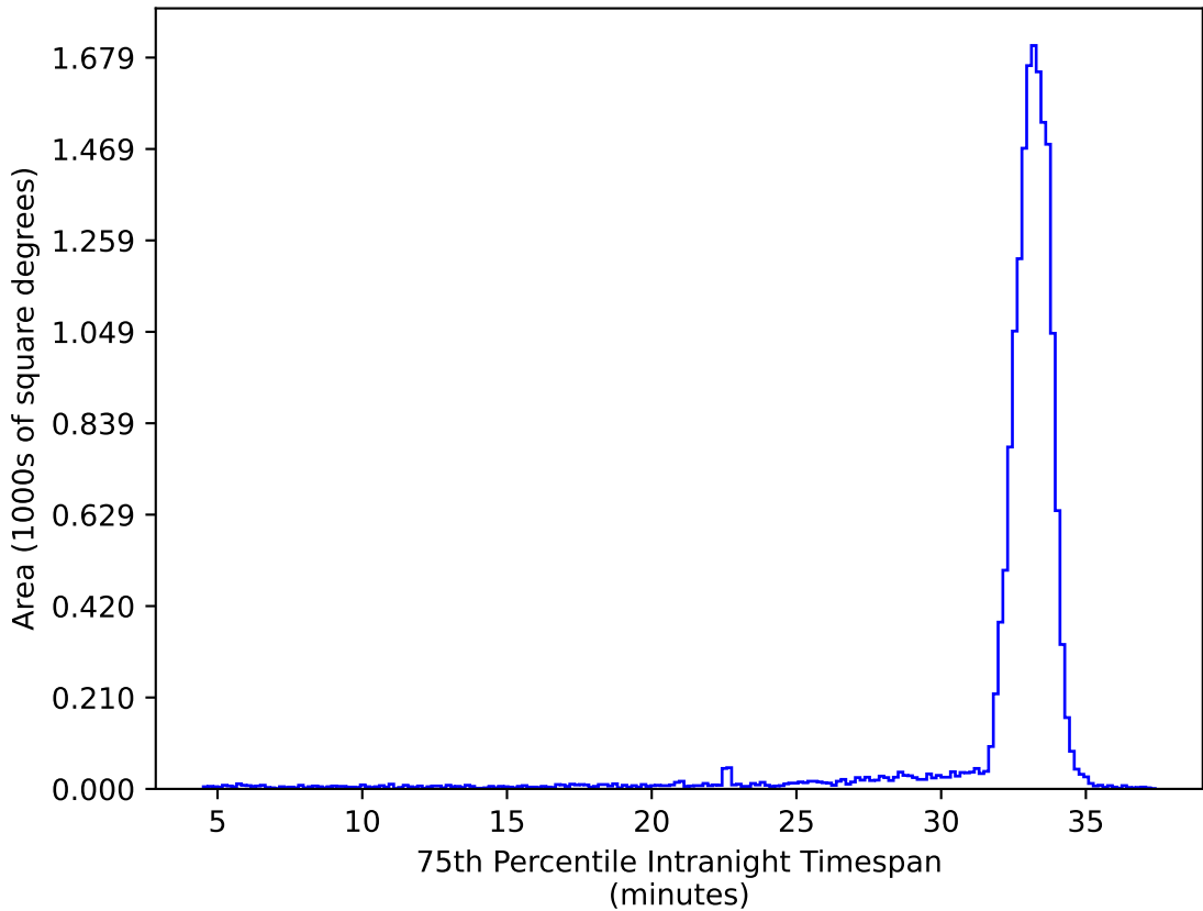
ddf_half_v3.4_10yrs WFD ug bands: 75th Percentile Intranight Timespan
