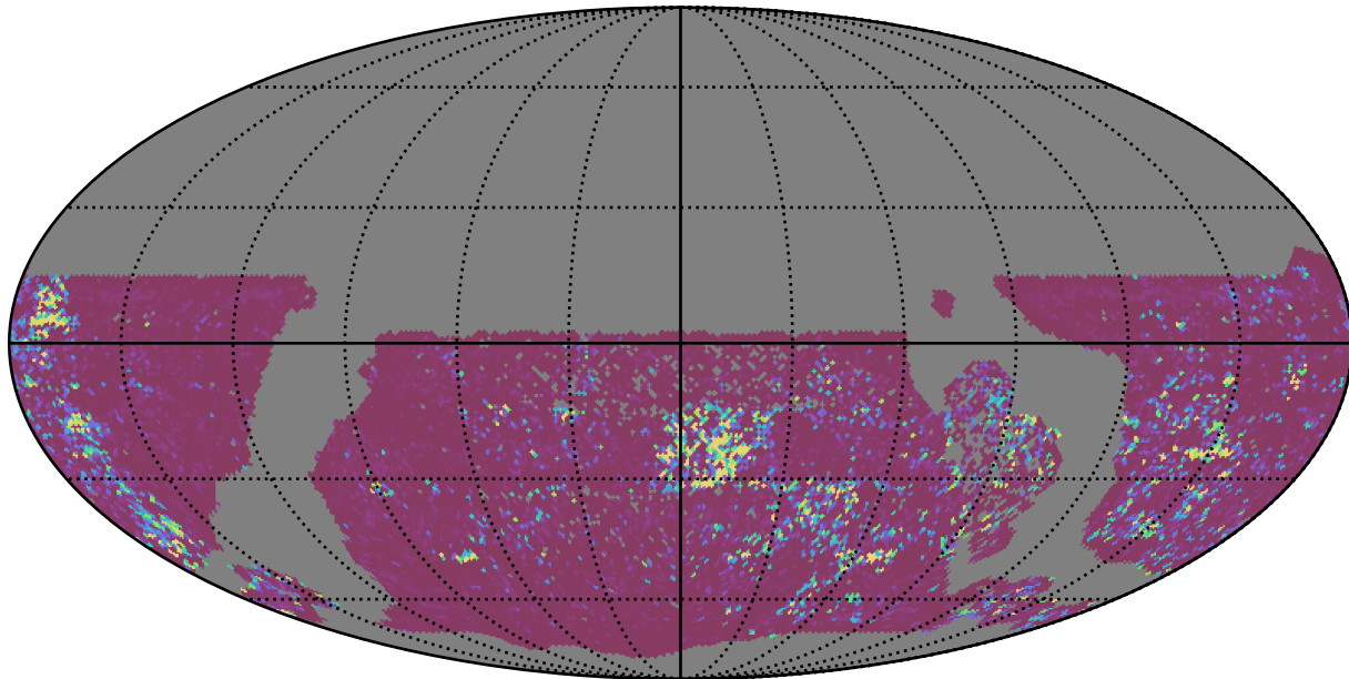
ddf_half_v3.4_10yrs WFD u band: 75th Percentile Intranight Timespan
