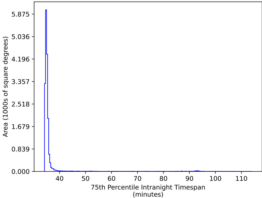
ddf_half_v3.4_10yrs WFD ri bands: 75th Percentile Intranight Timespan
