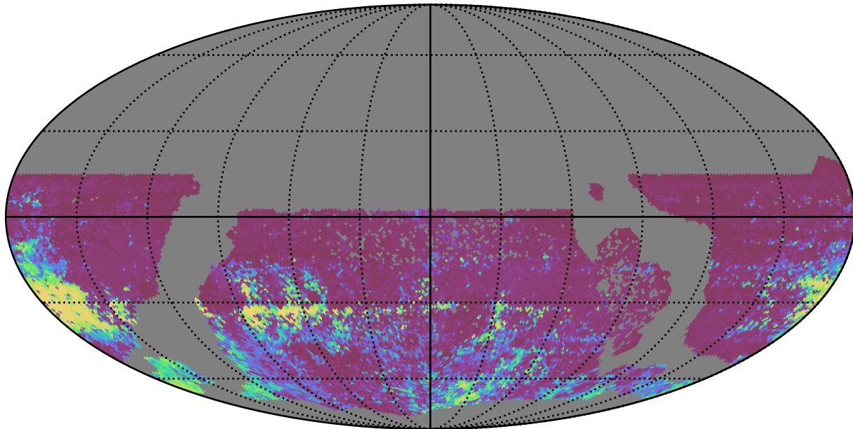
ddf_half_v3.4_10yrs WFD r band: 75th Percentile Intranight Timespan
