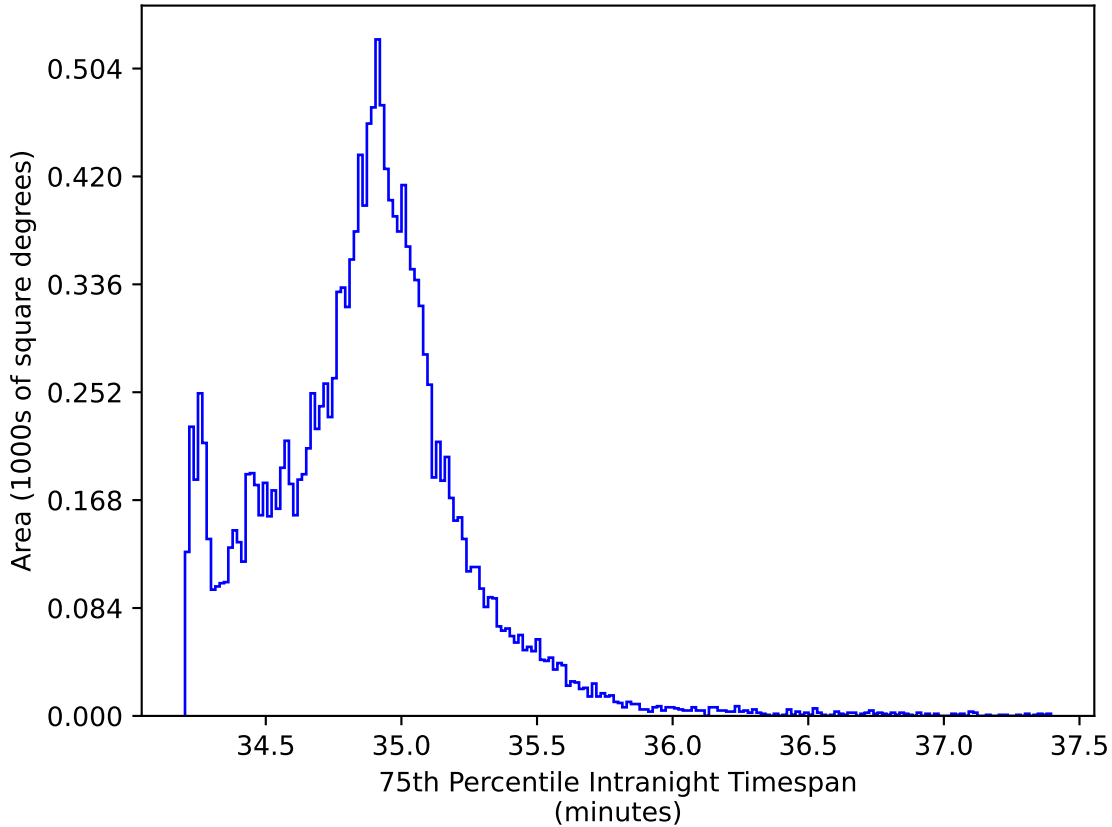
ddf_half_v3.4_10yrs WFD iz bands: 75th Percentile Intranight Timespan
