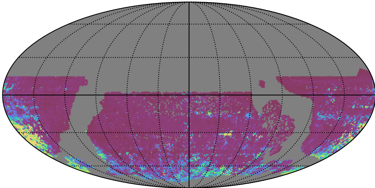
ddf_half_v3.4_10yrs WFD i band: 75th Percentile Intranight Timespan
