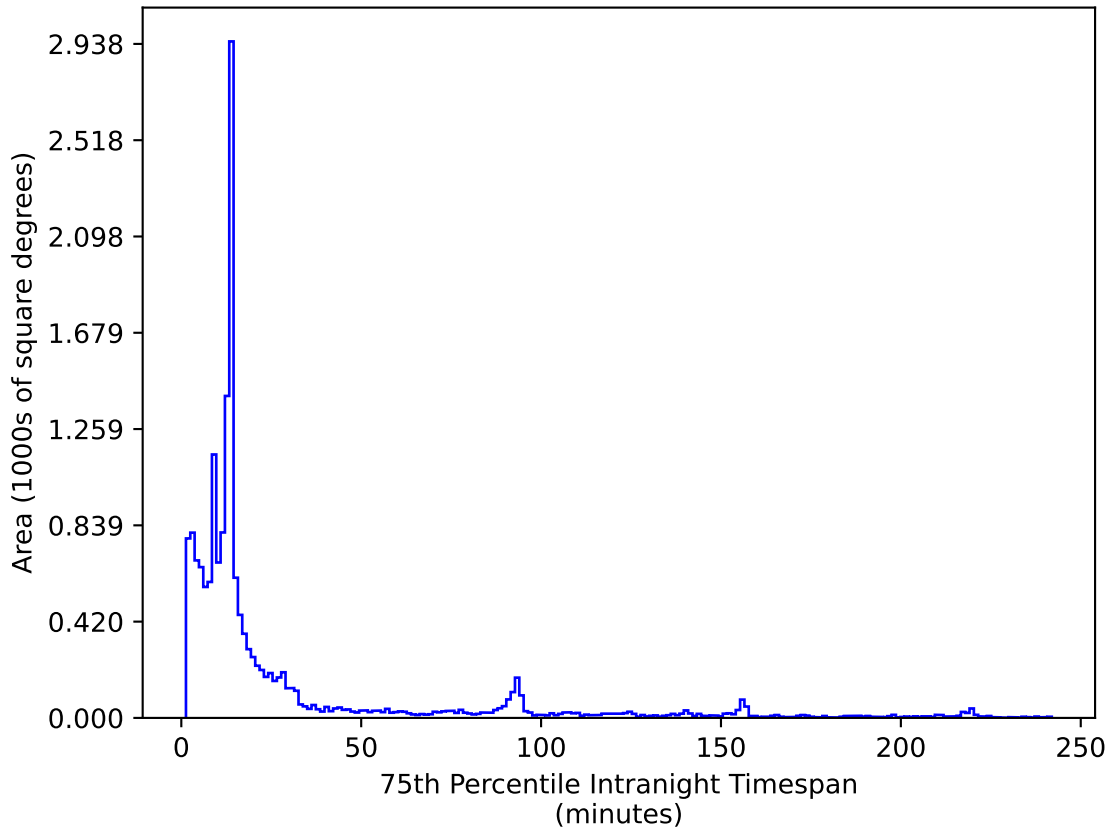
ddf_half_v3.4_10yrs WFD i band: 75th Percentile Intranight Timespan
