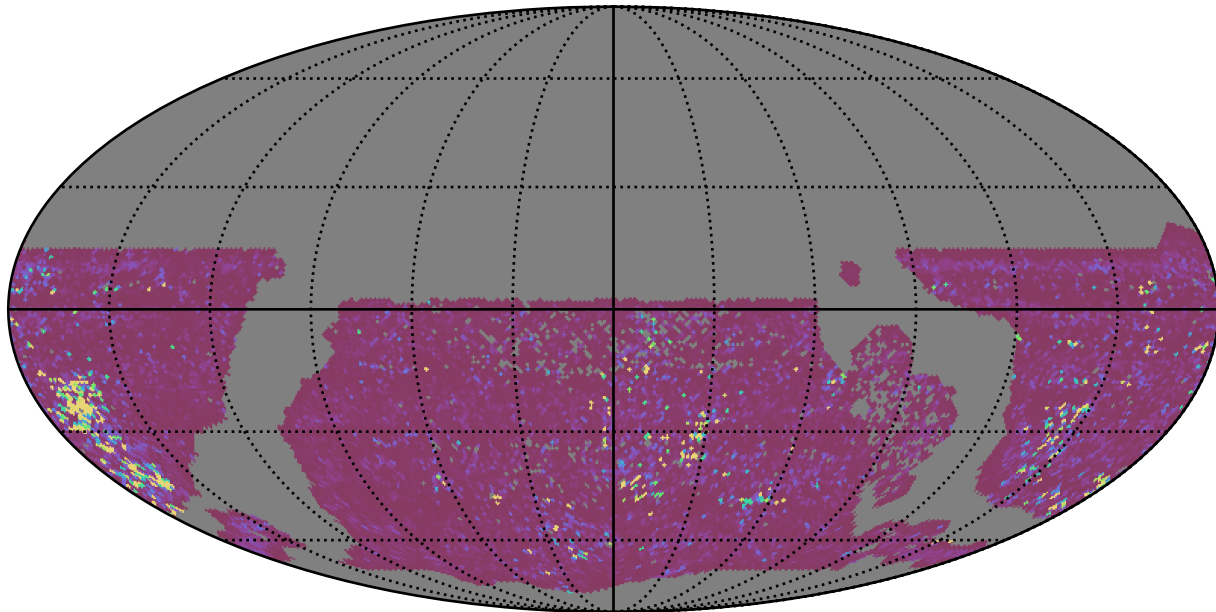
ddf_half_v3.4_10yrs WFD g band: 75th Percentile Intranight Timespan
