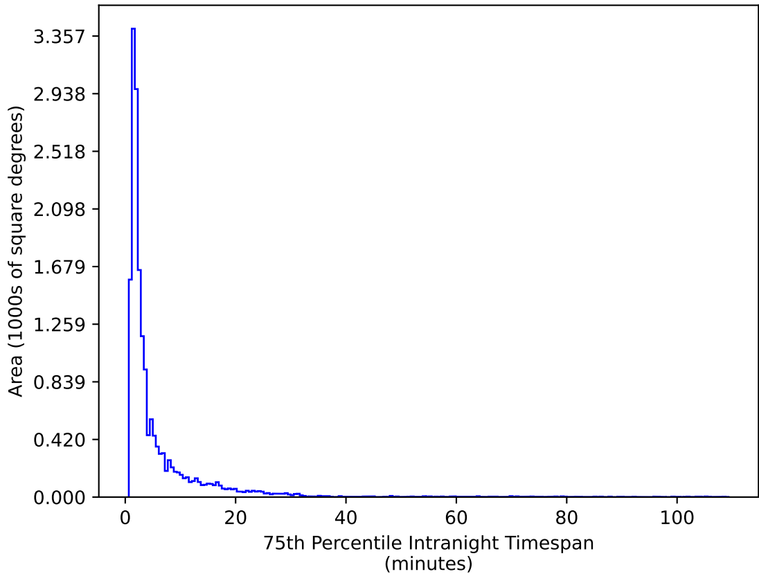
ddf_half_v3.4_10yrs WFD g band: 75th Percentile Intranight Timespan
