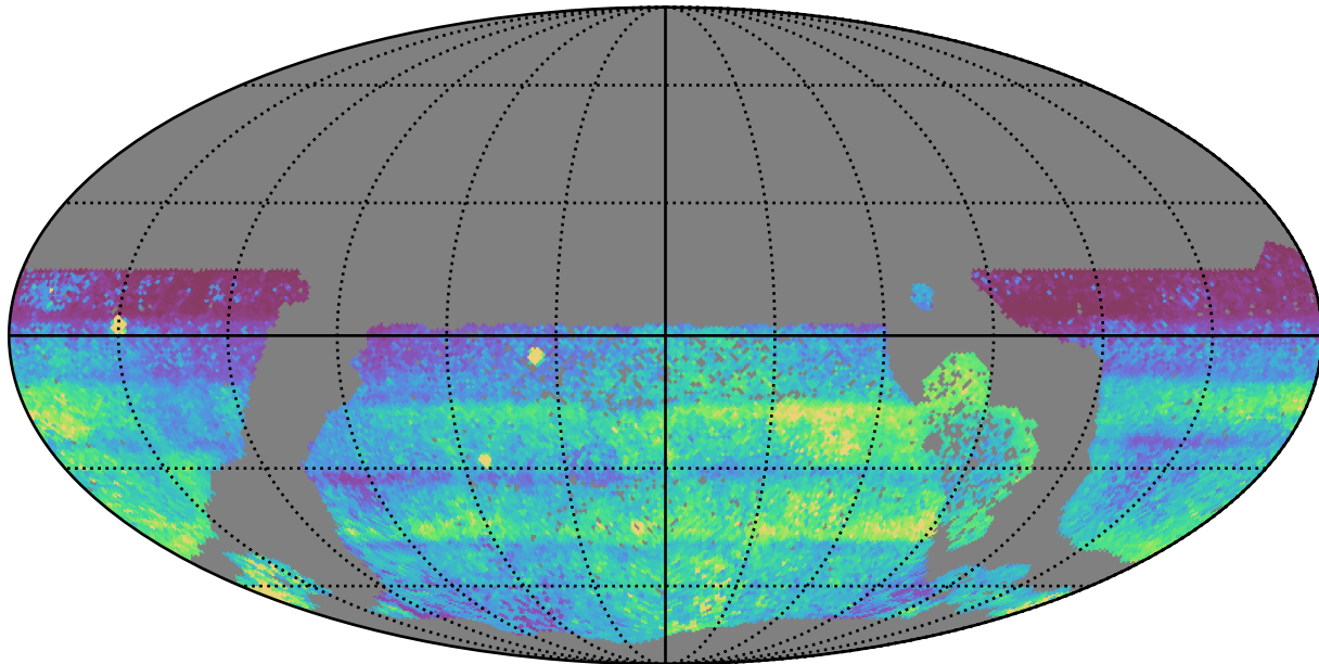
ddf_half_v3.4_10yrs WFD: 75th Percentile Intranight Timespan
