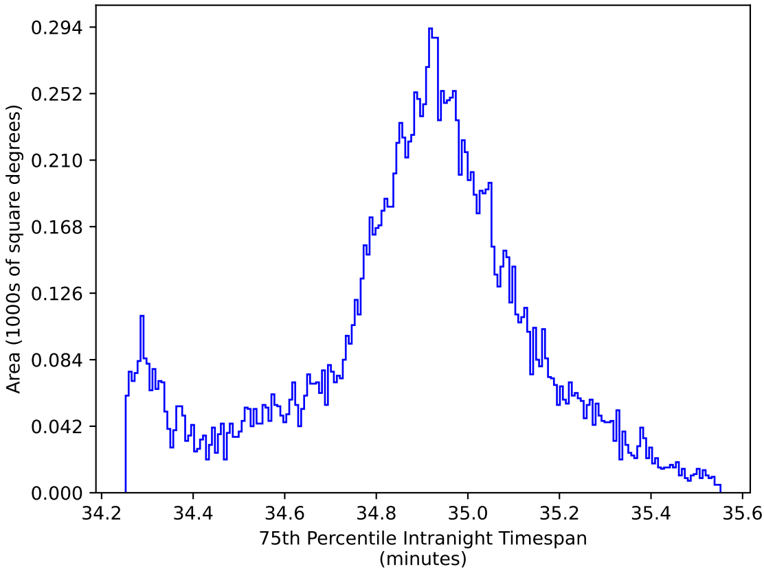
ddf_half_v3.4_10yrs WFD: 75th Percentile Intranight Timespan
