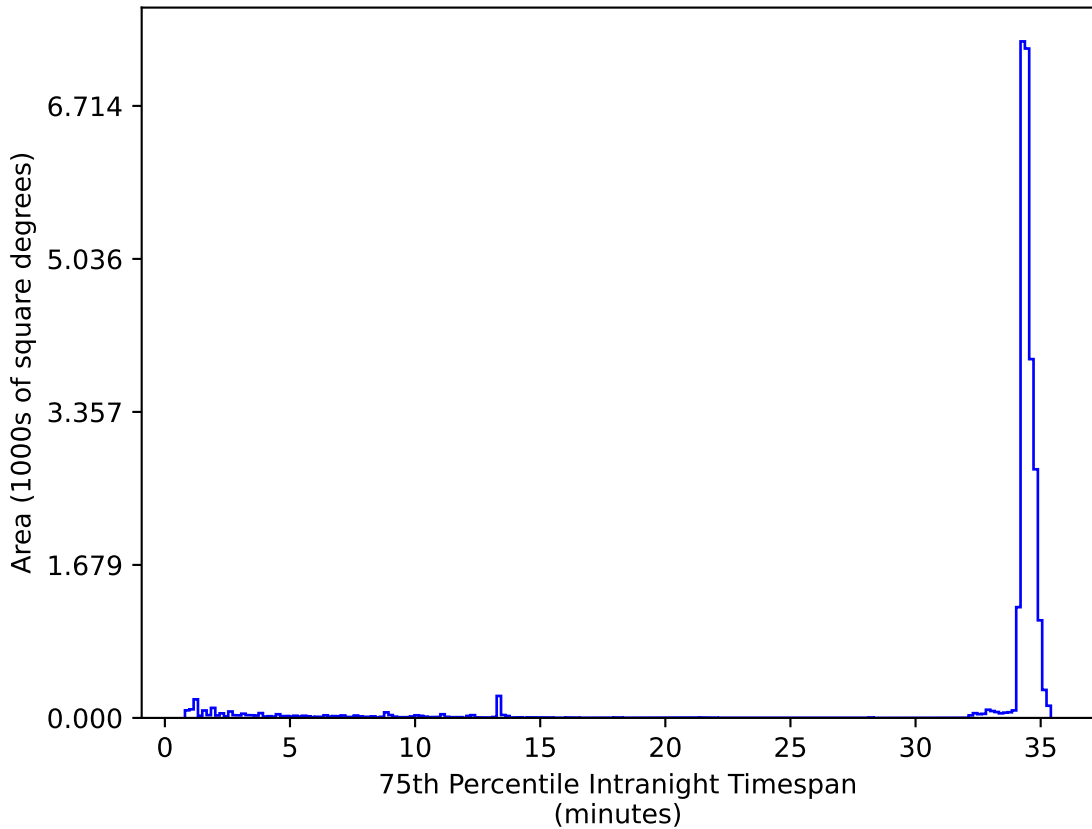
ddf_half_v3.4_10yrs All sky zy bands: 75th Percentile Intranight Timespan
