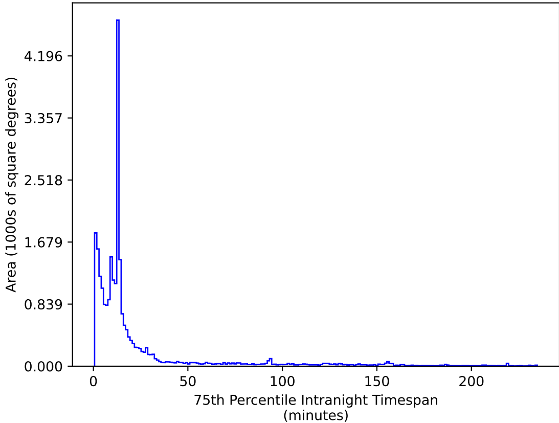
ddf_half_v3.4_10yrs All sky z band: 75th Percentile Intranight Timespan
