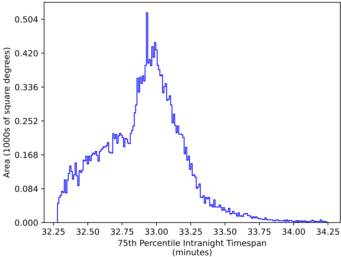
ddf_half_v3.4_10yrs All sky y band: 75th Percentile Intranight Timespan
