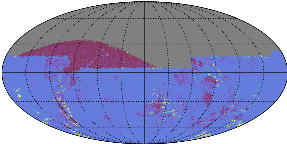
ddf_half_v3.4_10yrs All sky ug bands: 75th Percentile Intranight Timespan
