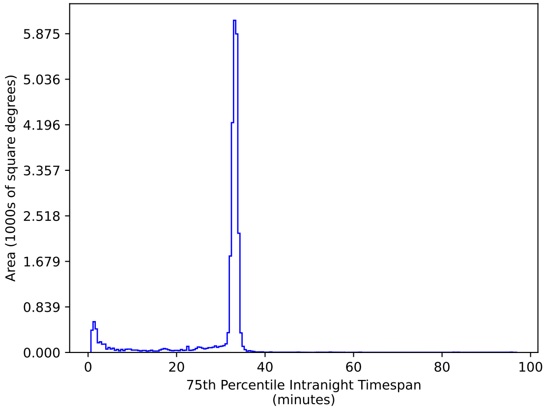
ddf_half_v3.4_10yrs All sky ug bands: 75th Percentile Intranight Timespan
