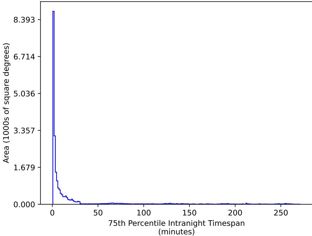
ddf_half_v3.4_10yrs All sky u band: 75th Percentile Intranight Timespan
