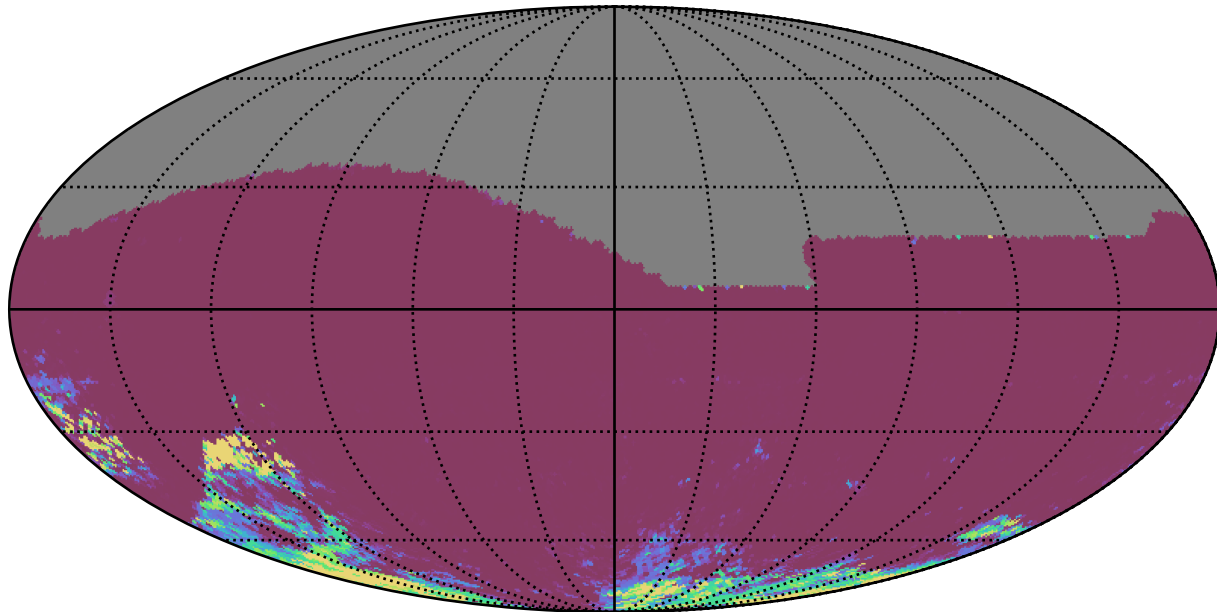
ddf_half_v3.4_10yrs All sky ri bands: 75th Percentile Intranight Timespan
