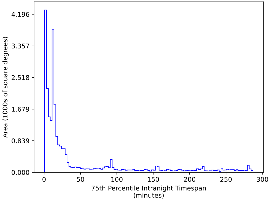
ddf_half_v3.4_10yrs All sky r band: 75th Percentile Intranight Timespan
