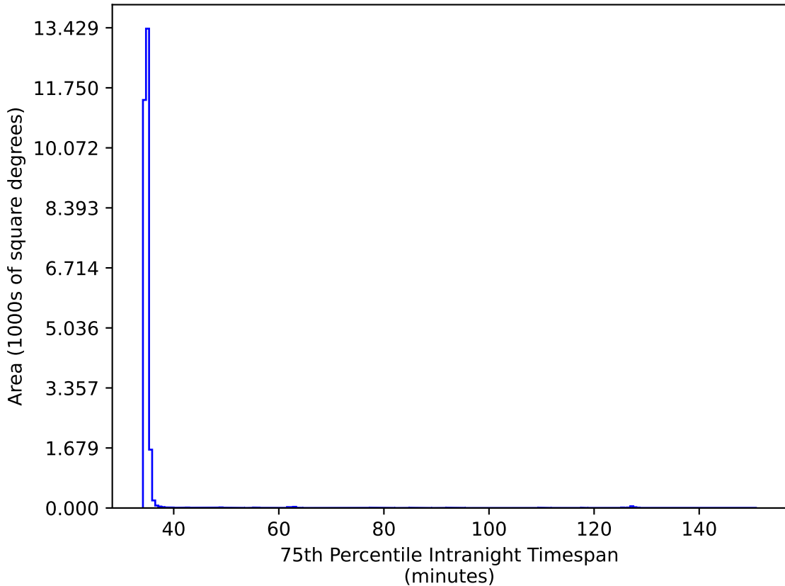
ddf_half_v3.4_10yrs All sky iz bands: 75th Percentile Intranight Timespan
