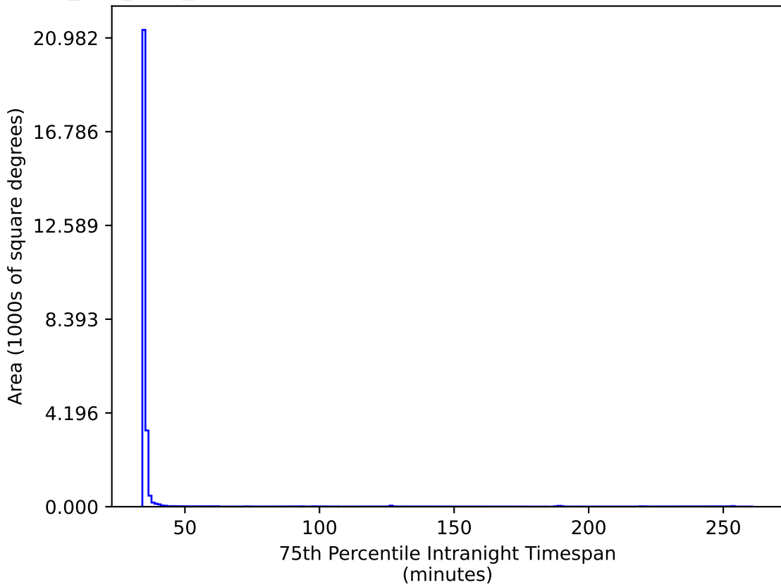
ddf_half_v3.4_10yrs All sky gr bands: 75th Percentile Intranight Timespan
