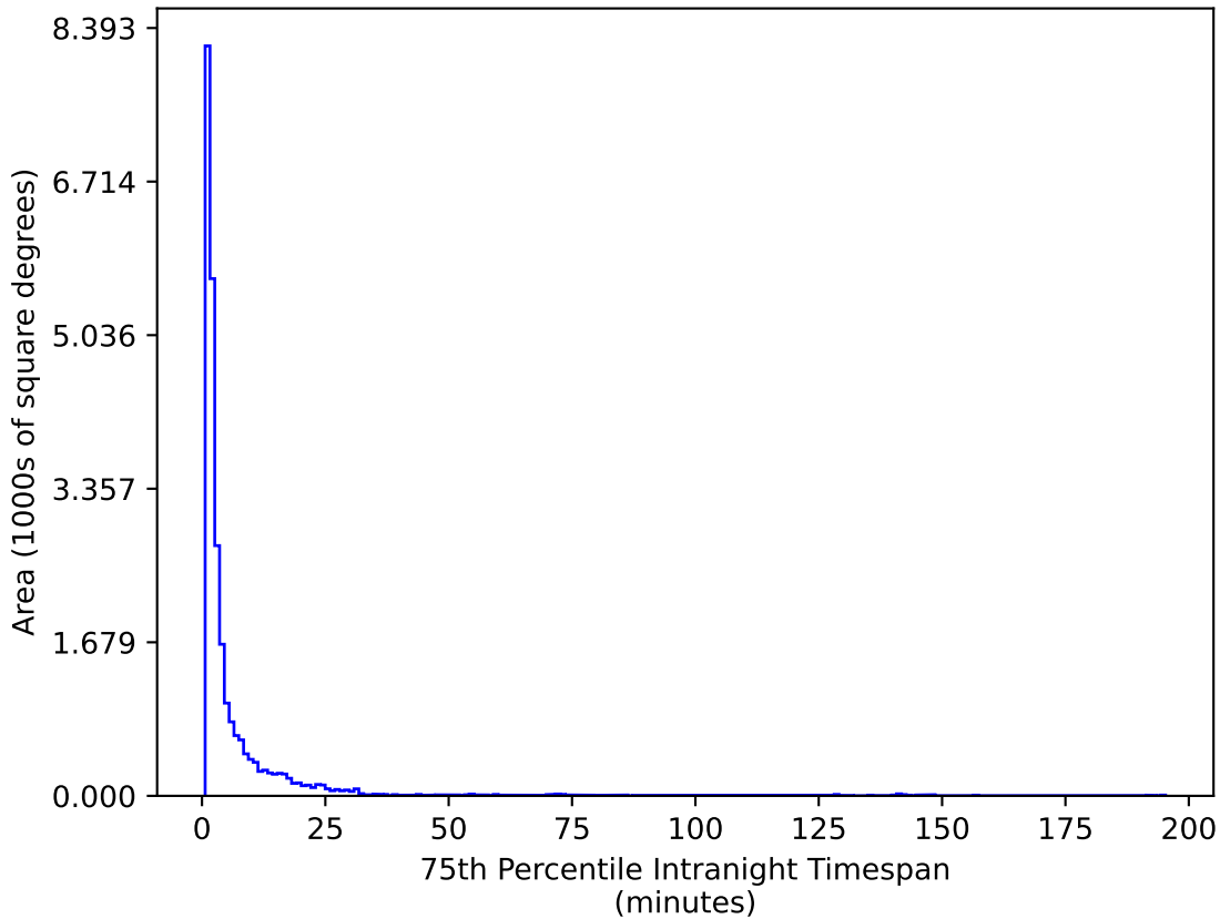
ddf_half_v3.4_10yrs All sky g band: 75th Percentile Intranight Timespan
