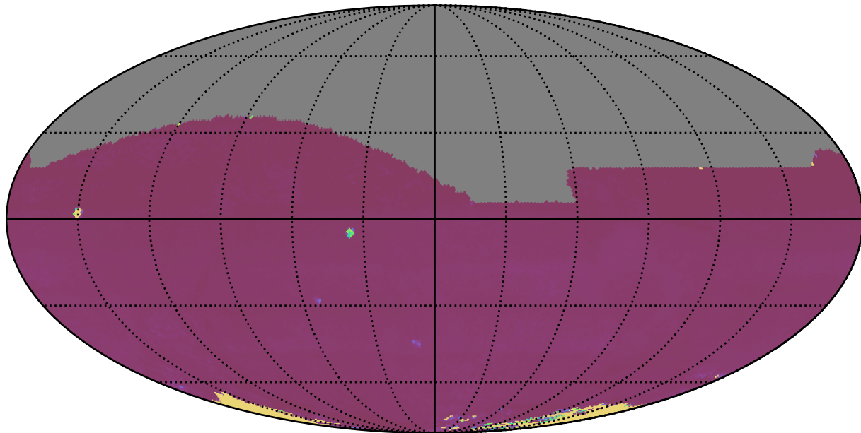
ddf_half_v3.4_10yrs All sky all bands: 75th Percentile Intranight Timespan
