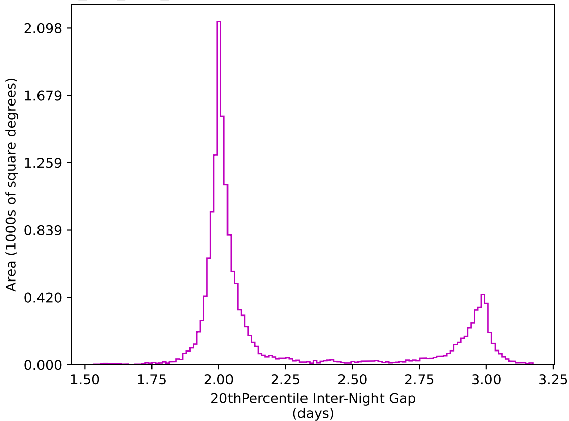
ddf_half_v3.4_10yrs WFD z band: 20thPercentile Inter-Night Gap
