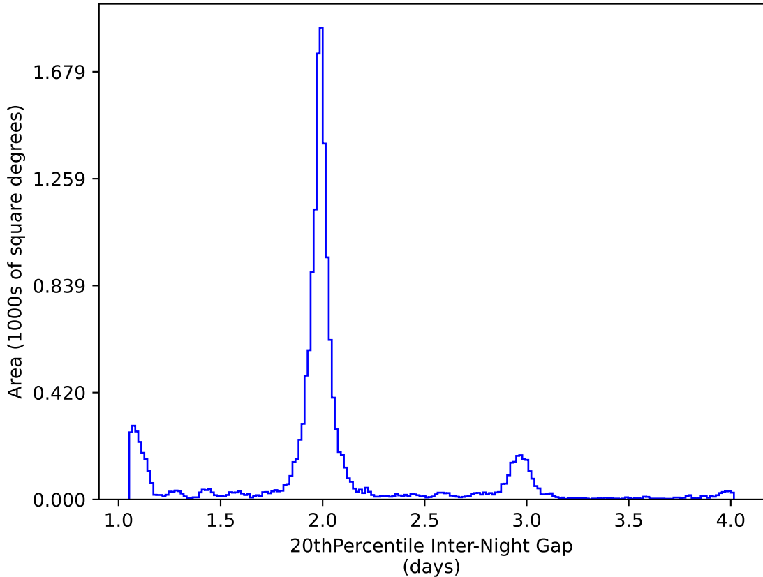
ddf_half_v3.4_10yrs WFD y band: 20thPercentile Inter-Night Gap
