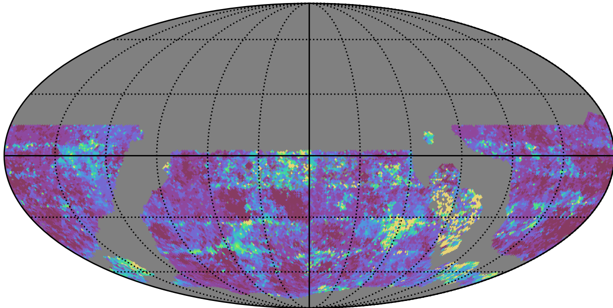
ddf_half_v3.4_10yrs WFD u band: 20thPercentile Inter-Night Gap
