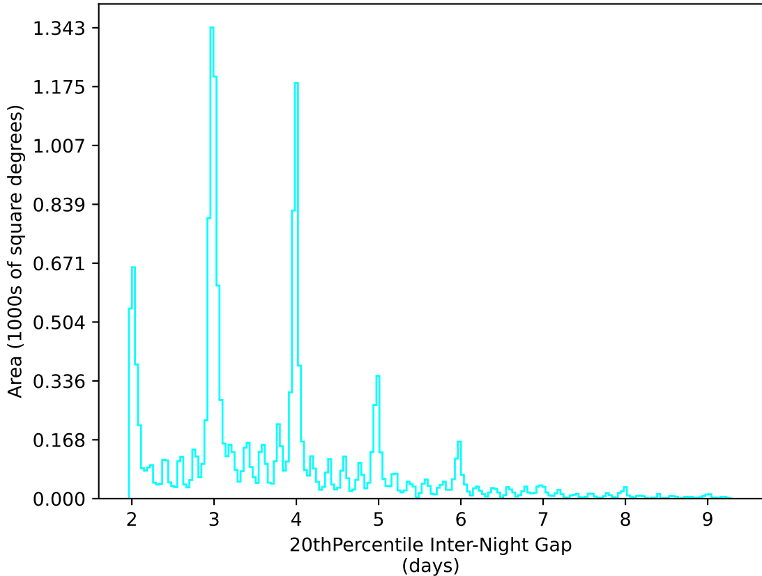
ddf_half_v3.4_10yrs WFD u band: 20thPercentile Inter-Night Gap
