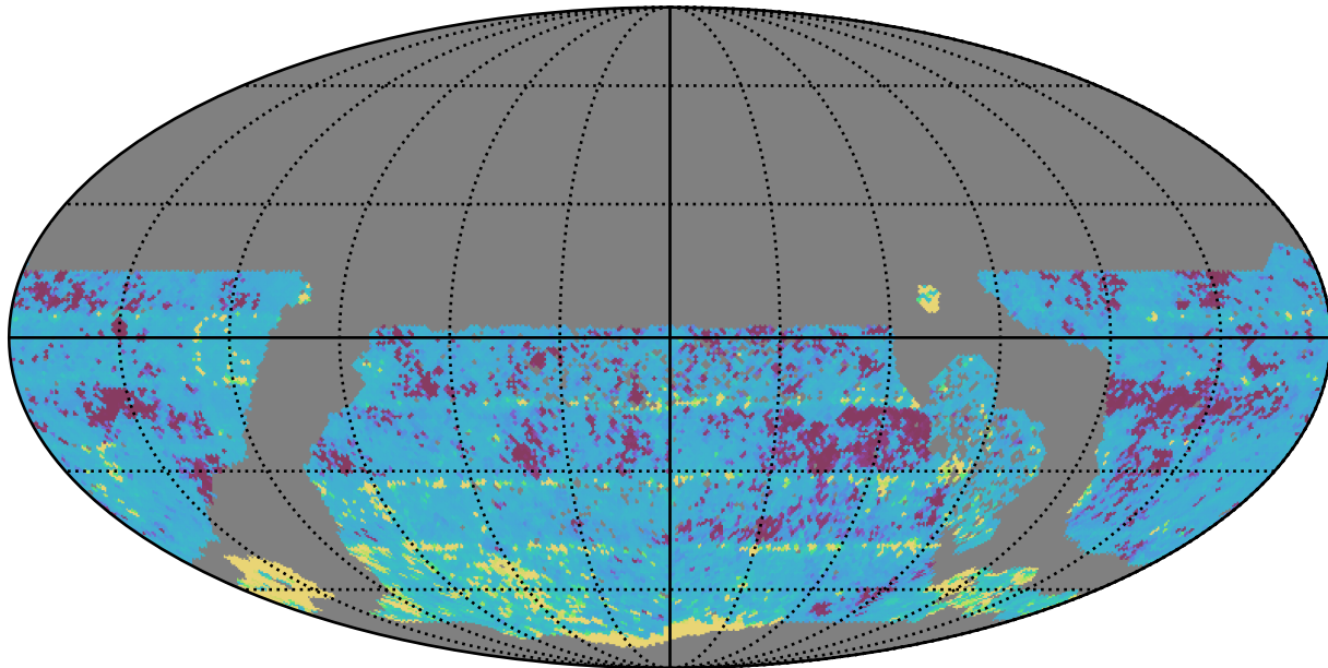
ddf_half_v3.4_10yrs WFD r band: 20thPercentile Inter-Night Gap
