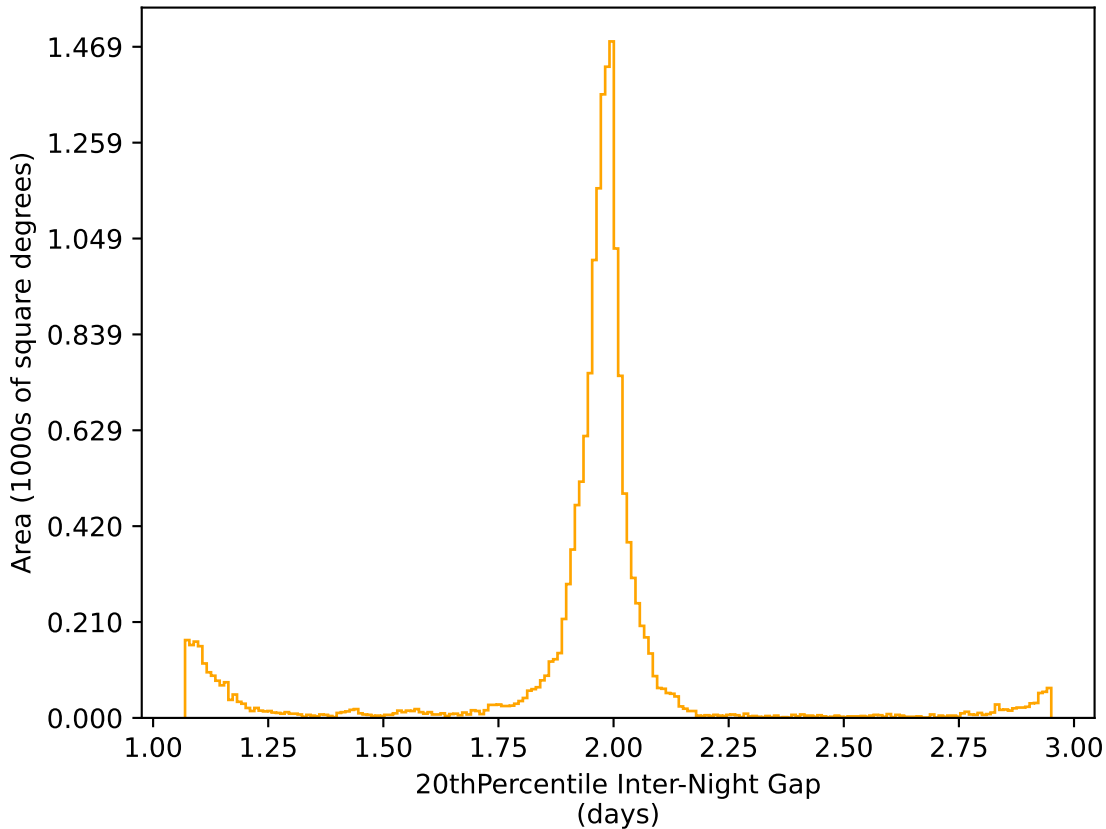
ddf_half_v3.4_10yrs WFD r band: 20thPercentile Inter-Night Gap
