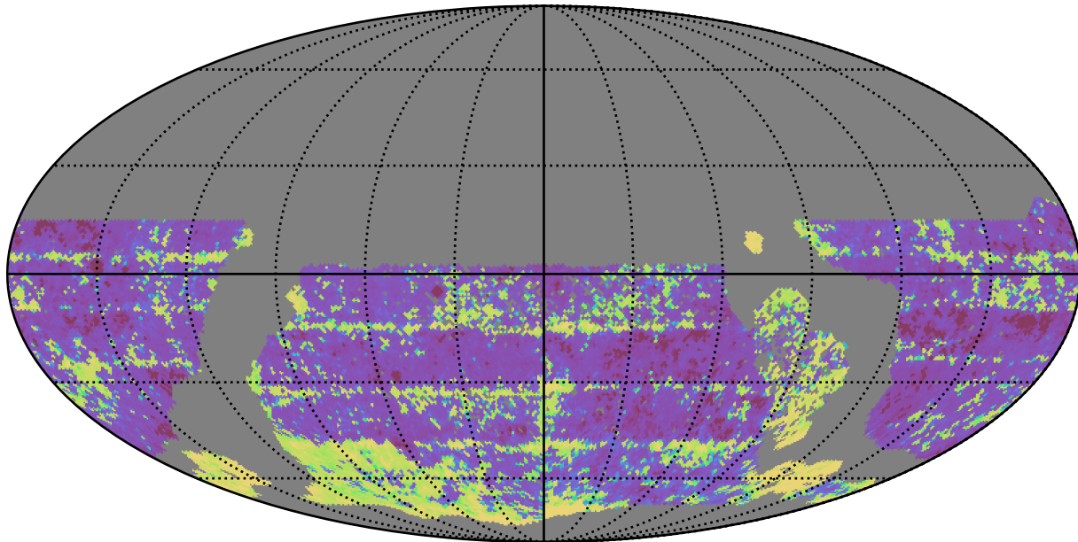
ddf_half_v3.4_10yrs WFD i band: 20thPercentile Inter-Night Gap
