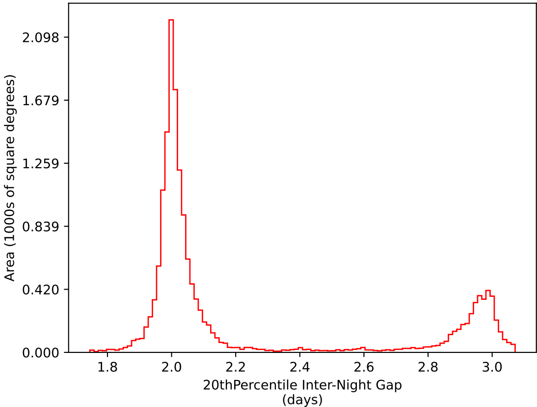
ddf_half_v3.4_10yrs WFD i band: 20thPercentile Inter-Night Gap
