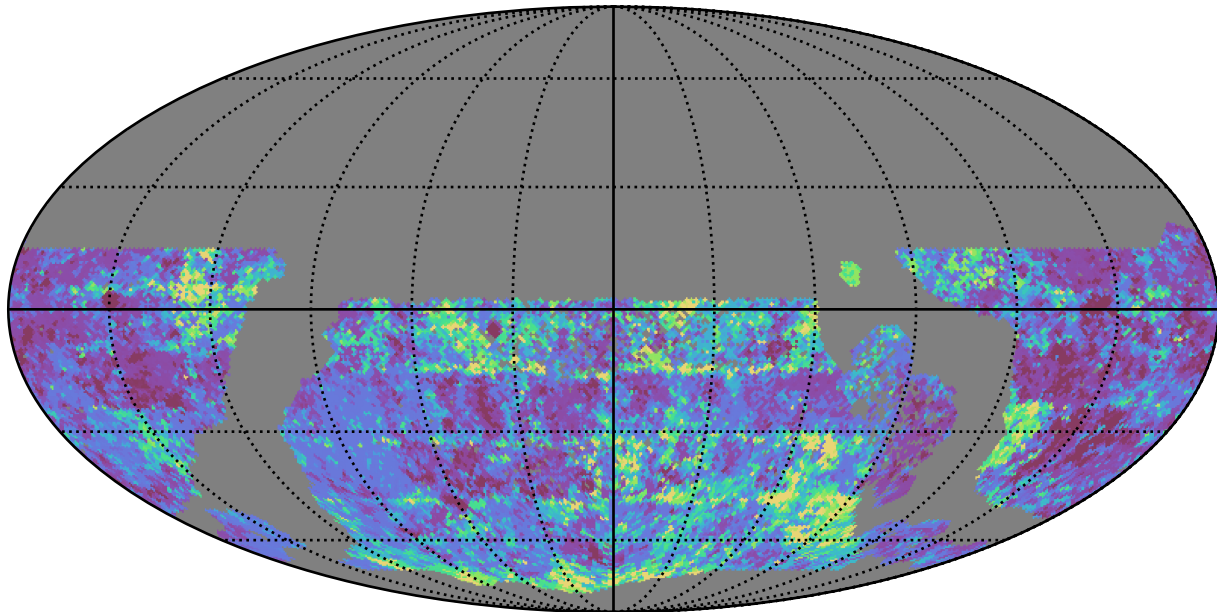
ddf_half_v3.4_10yrs WFD g band: 20thPercentile Inter-Night Gap
