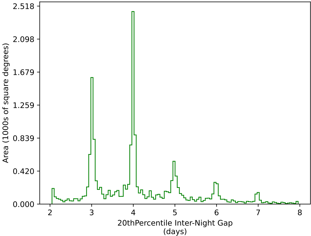
ddf_half_v3.4_10yrs WFD g band: 20thPercentile Inter-Night Gap
