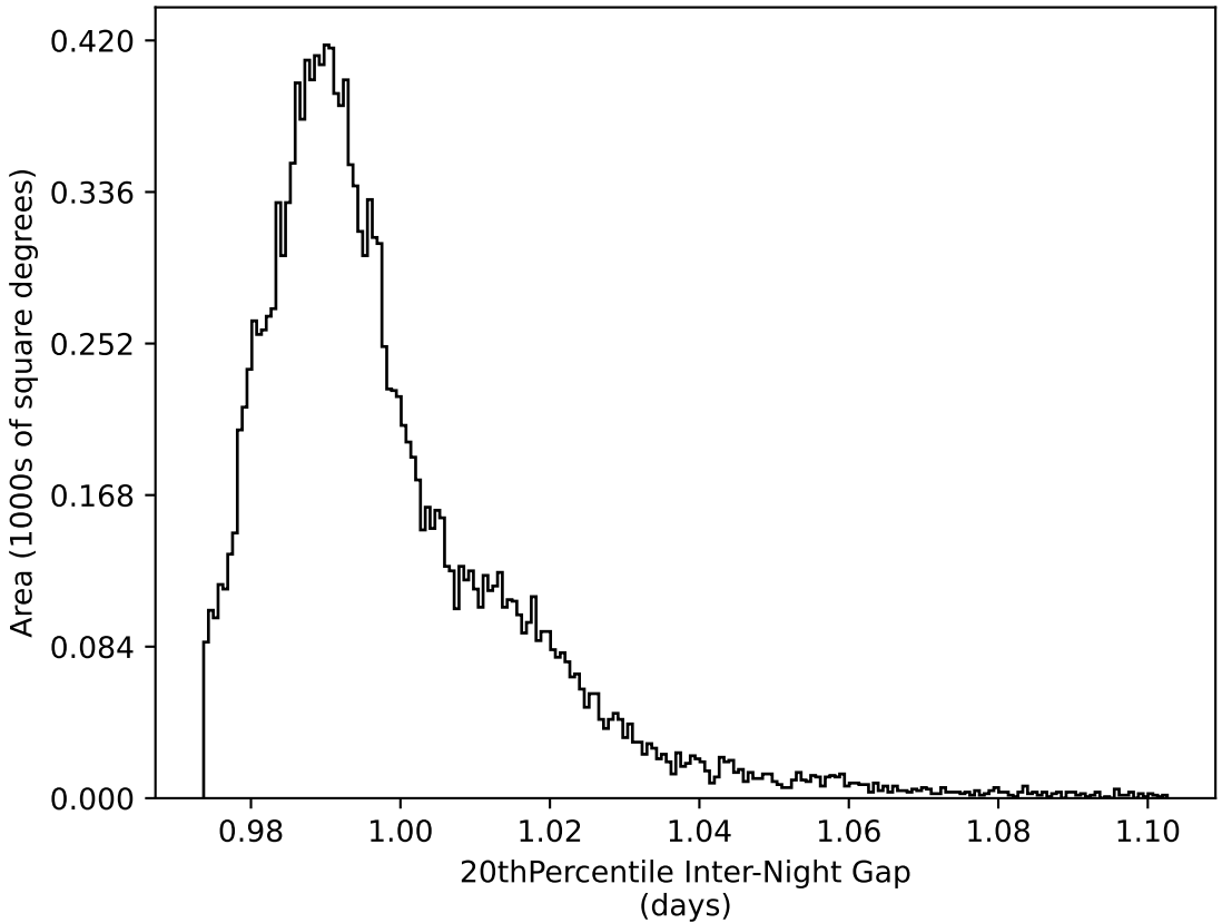
ddf_half_v3.4_10yrs WFD all bands: 20thPercentile Inter-Night Gap
