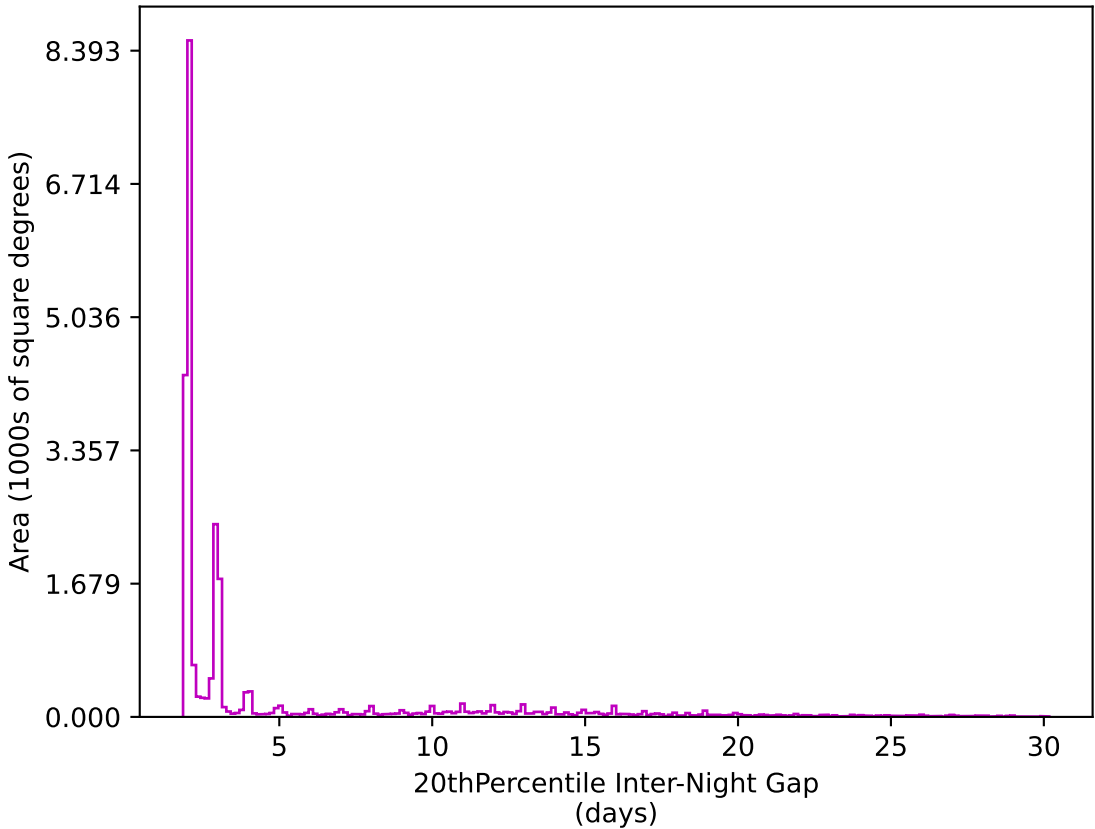
ddf_half_v3.4_10yrs All sky z band: 20thPercentile Inter-Night Gap
