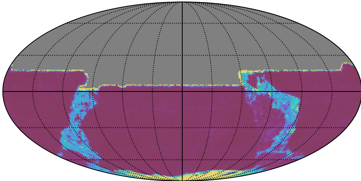
ddf_half_v3.4_10yrs All sky y band: 20thPercentile Inter-Night Gap
