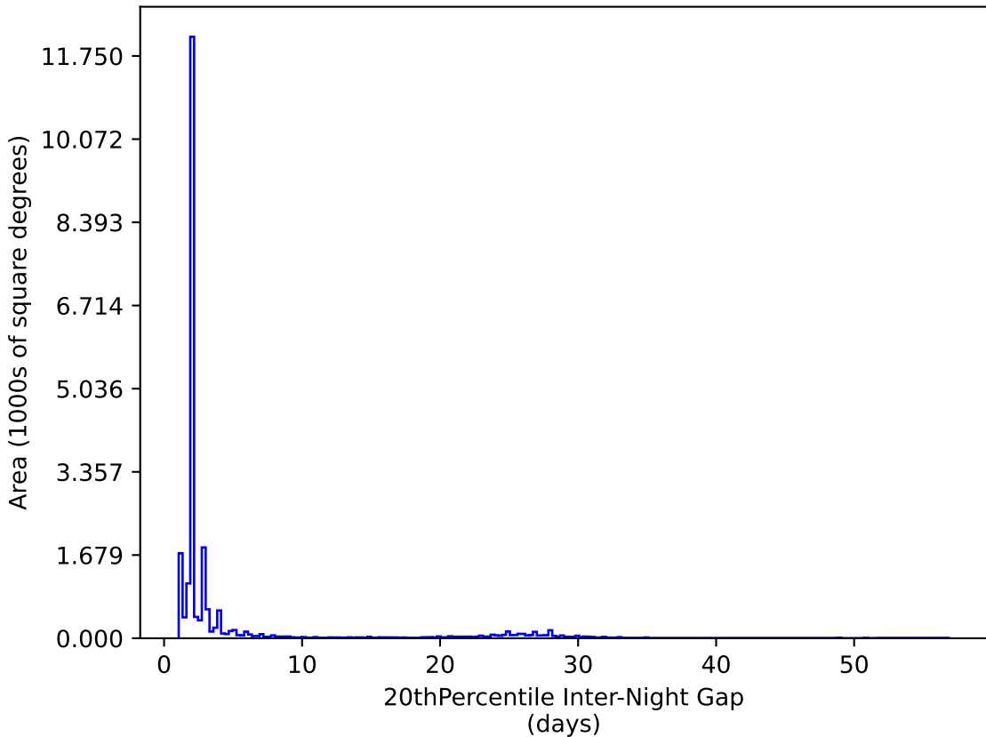
ddf_half_v3.4_10yrs All sky y band: 20thPercentile Inter-Night Gap
