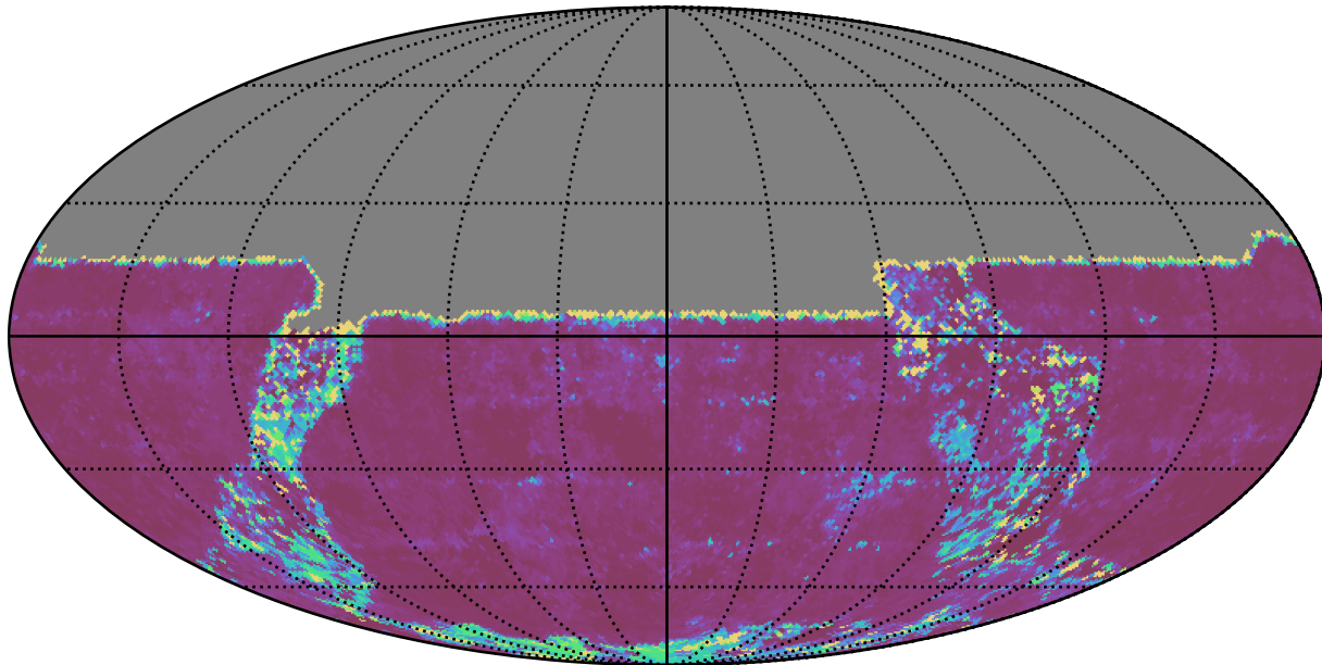
ddf_half_v3.4_10yrs All sky u band: 20thPercentile Inter-Night Gap
