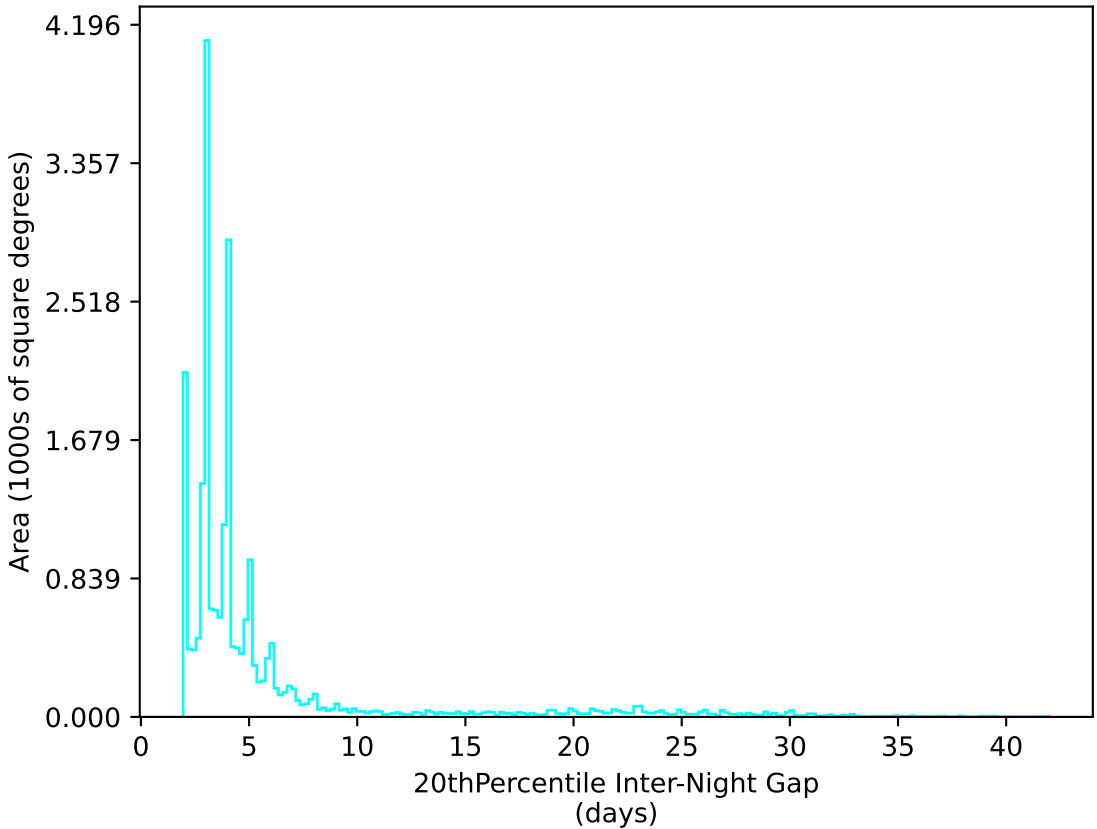
ddf_half_v3.4_10yrs All sky u band: 20thPercentile Inter-Night Gap
